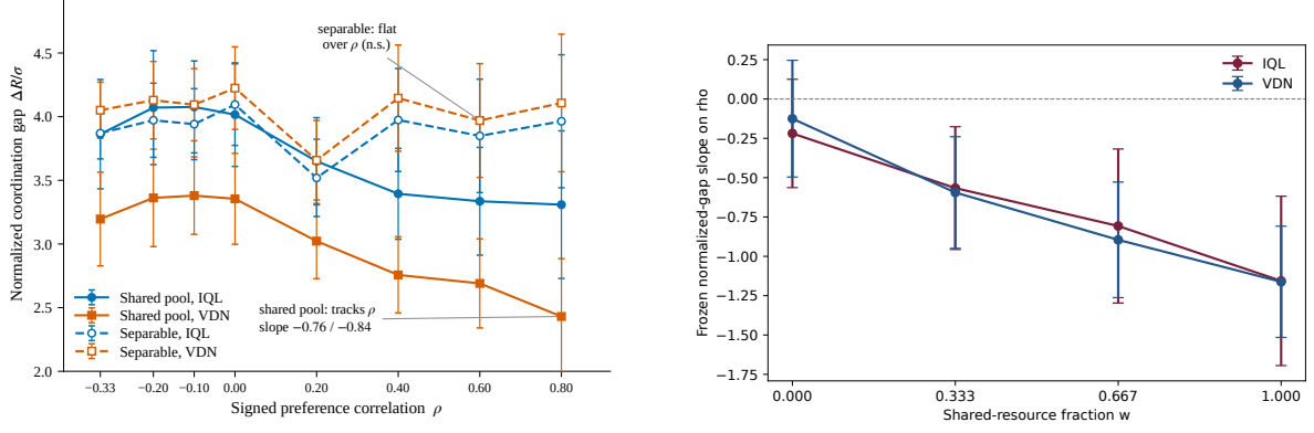
Figure 2: Interaction-structure scope and overlap response on legacy-Gaussian-at-zero target support. Left: the signed gradient appears with shared state; the separable IQL expectation is \rho -invariant and the VDN slope is not detected. Right: on clean frozen held-out evaluation, the slope point estimates steepen over the four tested fixed first- k shared-coordinate configurations. Absolute levels are not compared across learners; error bars on the right are HC3 95% CIs.
